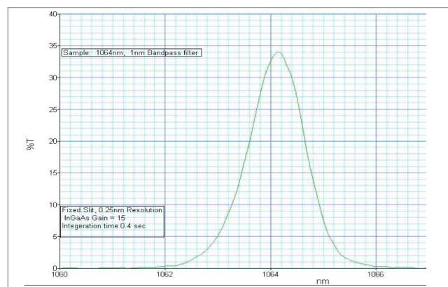
Figure 5. 1 nm Laser line filter measured with 0.25 nm resolution on a Lambda 1050 using an InGaAs detector.
