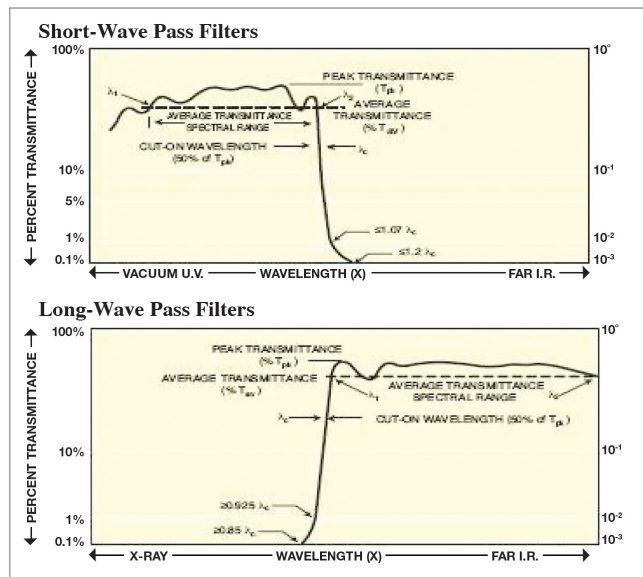
Figure 1. Typical filter design requirements.
