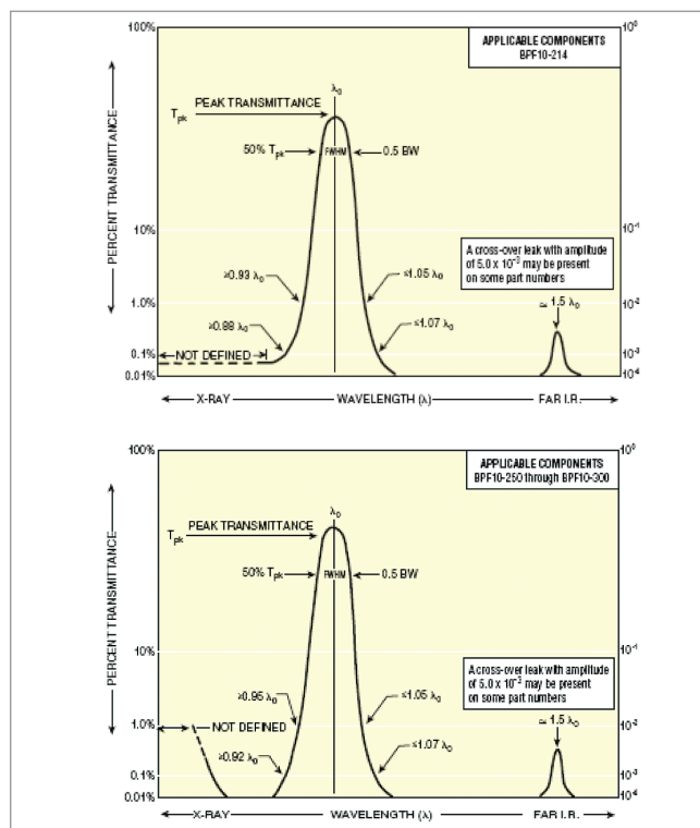
Figure 2. Typical bandpass filter response characteristics.
